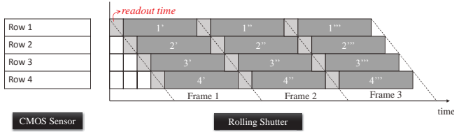
Fig. 2. Small delay exists between pixel rows due to the rolling shutter.
